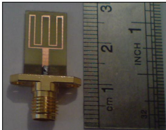
Fig 8. Photograph of the realized E-ring shaped monopole antenna.
