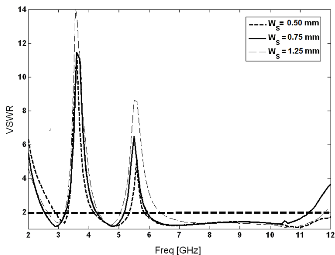
Fig. 7. Simulated VSWR characteristics for the proposed antenna with different values of W_s .
