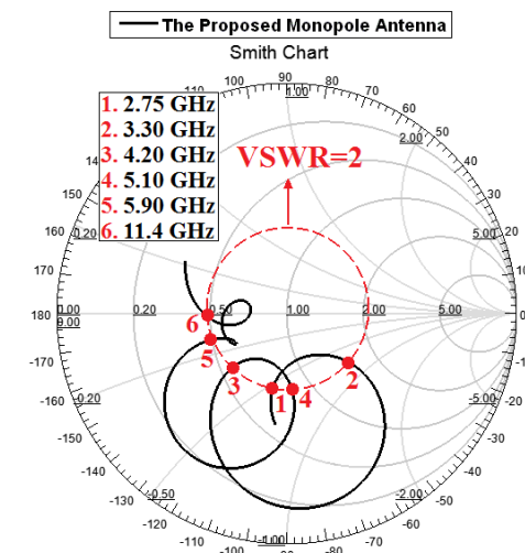
Fig.4. The simulated input impedance on a smith chart of the proposed E-ring shaped monopole antenna.
