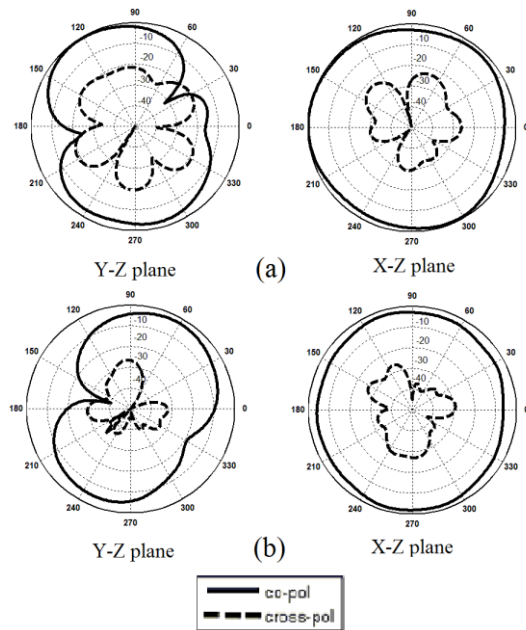
Fig 9. Measured radiation patterns of the proposed antenna (a) 4.7 GHz, (b) 9 GHz.
