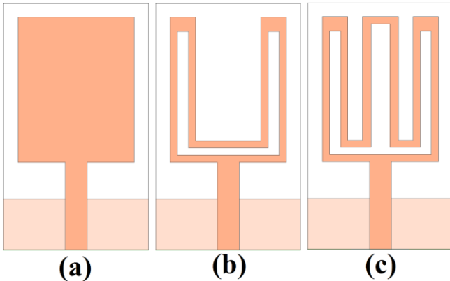
Fig. 2. (a) The ordinary Rectangular antenna, (b) the U-ring shaped structure in the radiating patch, (c) the proposed antenna structure.
