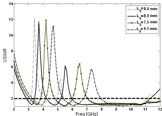
Fig. 6. Simulated VSWR characteristics for the proposed antenna with different values of L_s .
