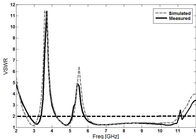
Fig. 9. Measured and simulated VSWR for the proposed antenna.
