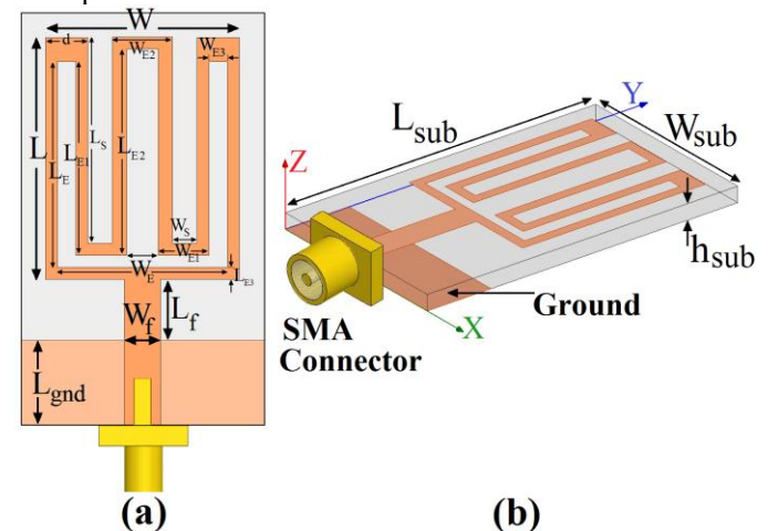
Fig. 1. Geometry of proposed E-ring shaped monopole antenna (a) top view, (b) side view.
