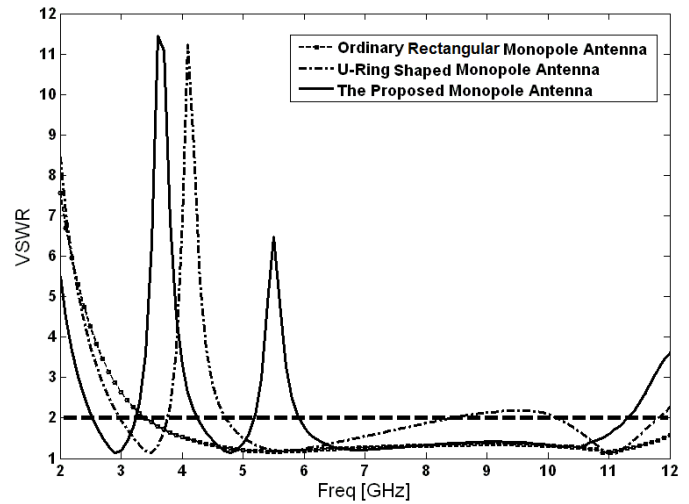
Fig. 3. Simulated VSWR characteristics for the antennas shown in Figure 2
